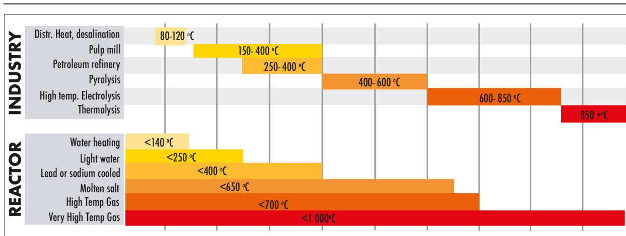
Temperature ranges used in various industries compared with temperature ranges produced by different types of reactors.
