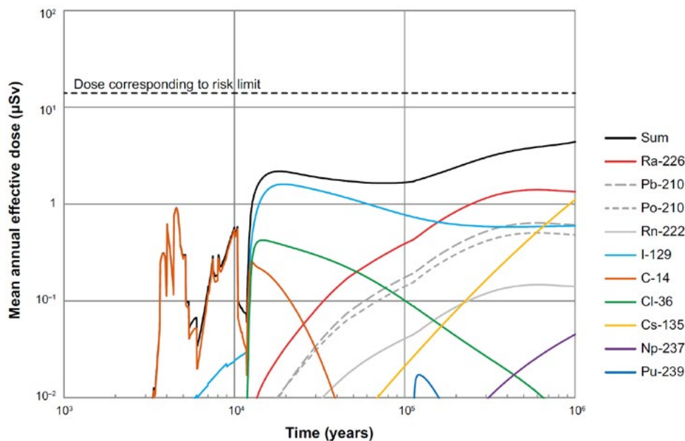
Figure 12: Consequences of “what-if” case. All waste canisters have a 4 mm hole through, and the buffer is gradually lost in the deposition holes with the highest groundwater flow rates. The maximum dose stays at around half of that allowed by regulations 85 .
