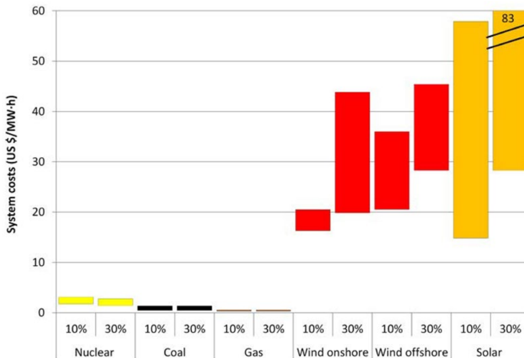
Figure 2: Ranges of system costs (backup, balancing, grid connection, reinforcement and extension) of selected technologies at their 10% and 30% shares in the grid in selected countries (Finland, France, Germany, Republic of Korea, United Kingdom and the USA). 44
