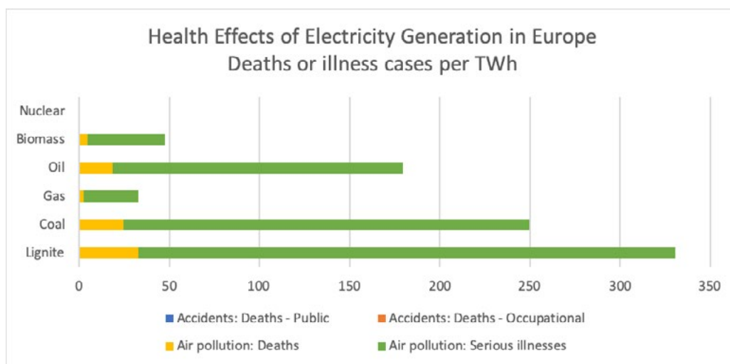
Figure 8: Deaths or illnesses per terawatt hours of electricity generation in Europe. Source: Lancet 2007 69
