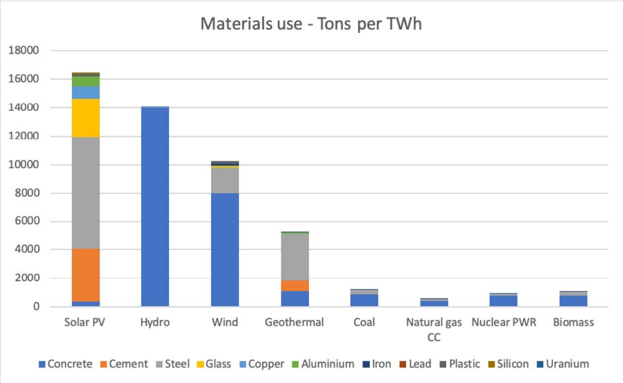
Figure 7: Materials use of energy production facilities - tons per TWh. Source: US DoE 2015. Uranium amount, 25 tons, added by authors.
