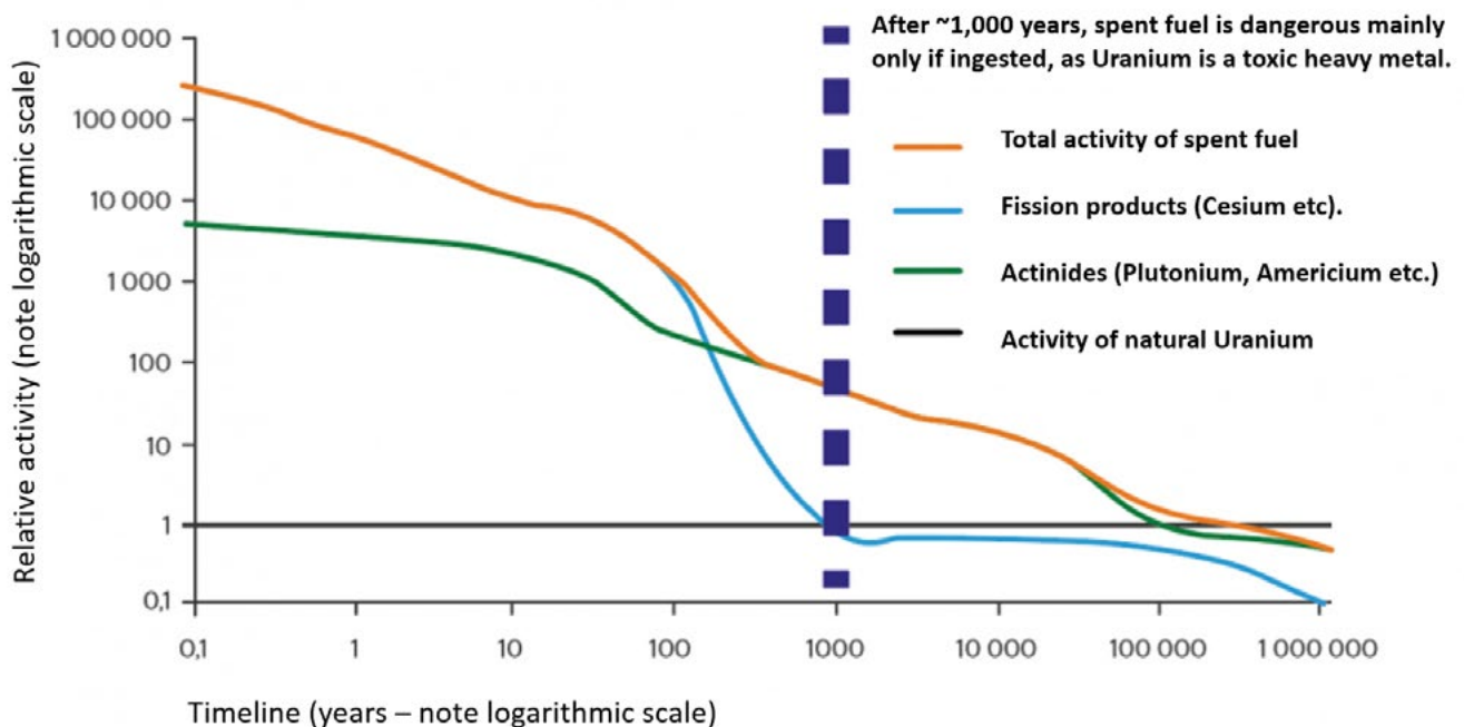
Figure 10: The development of spent nuclear fuel radioactive dose over time.
